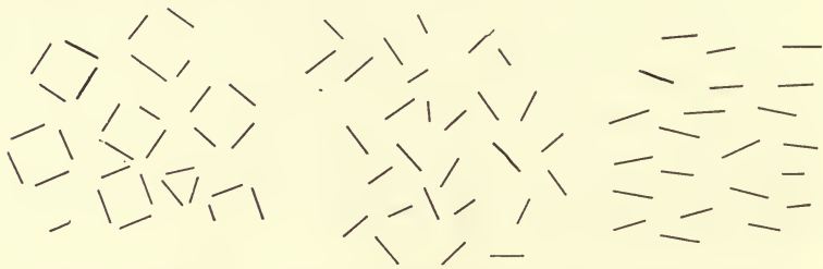
FIG. 27. Diagrams representing molecular magnets arranged in accordance with Ewing's theory of magnetism.
